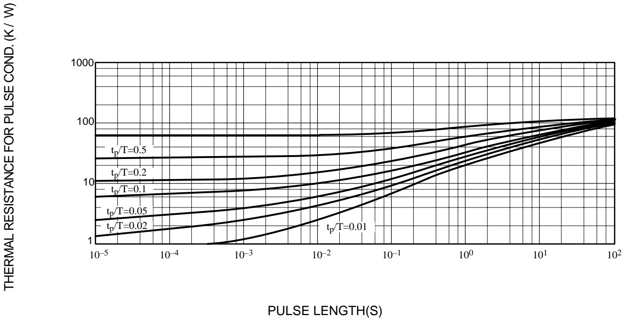
FIG.3 – THERMAL RESPONSE
