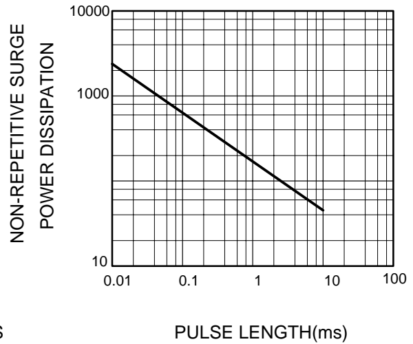
FIG.2 – NON REPETTIVE SURGE POWER DISSIPATION VS.PULSE LENGTH
